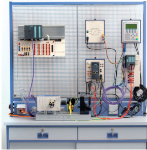
Training system "Profibus with PLC, motor and gear"
